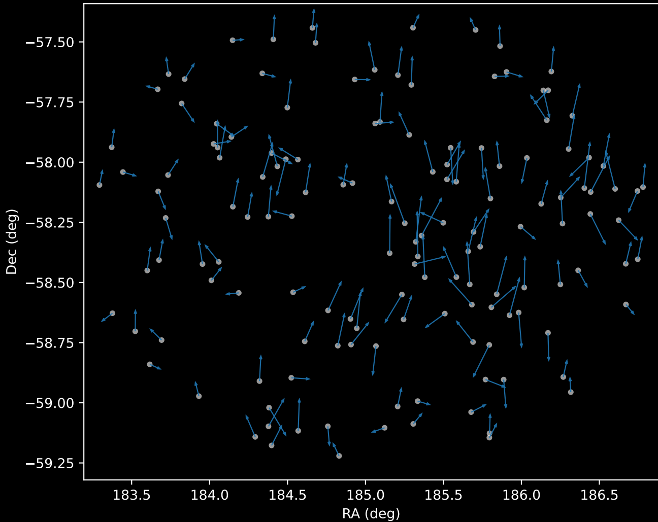
APOGEE DR17 Cluster 0 Proper Motion Vectors (n=143)
