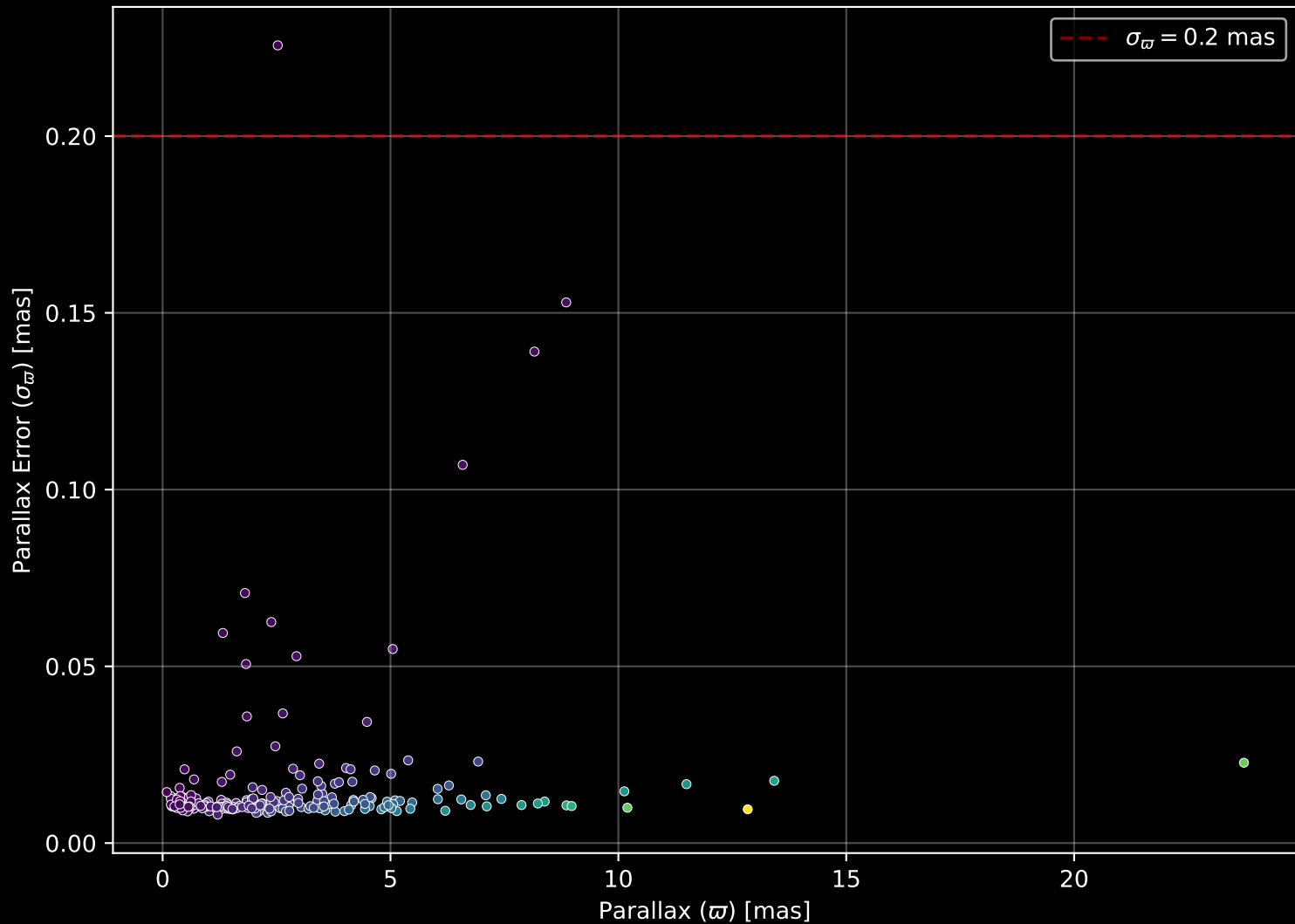
APOGEE DR17 Field: [267-32-O_TESS] Parallax Quality (n= 200)
