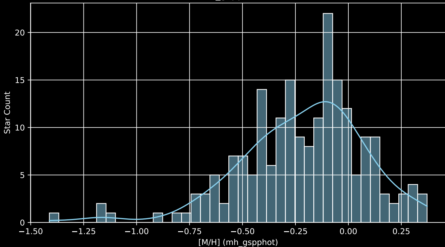
APOGEE DR17 Field: [267-32-O_TESS [M/H] (mh_gspphot) (n= 200)
