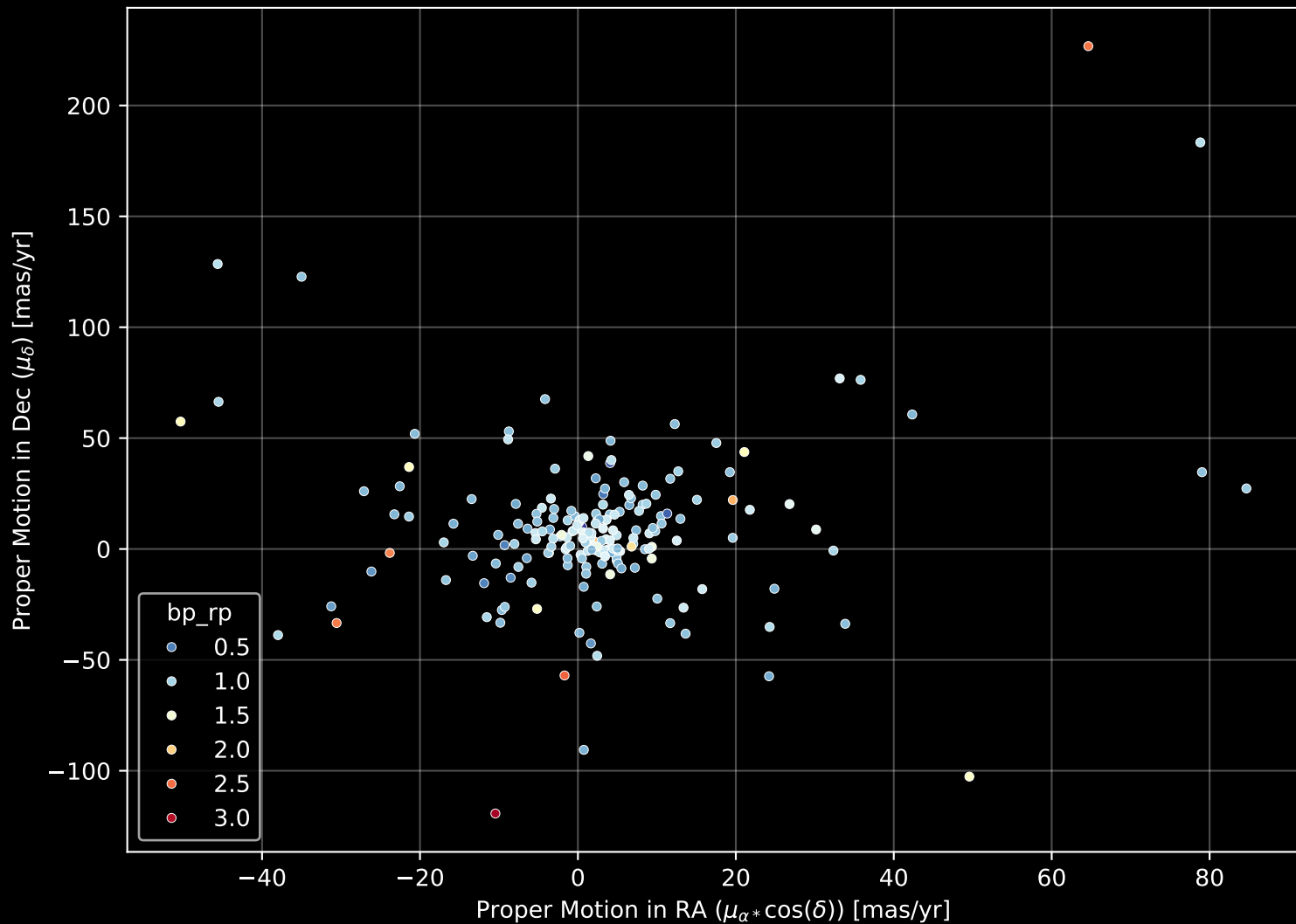
APOGEE DR17 Field: [267-32-O_TESS] Proper Motion Diagram (n= 200)
