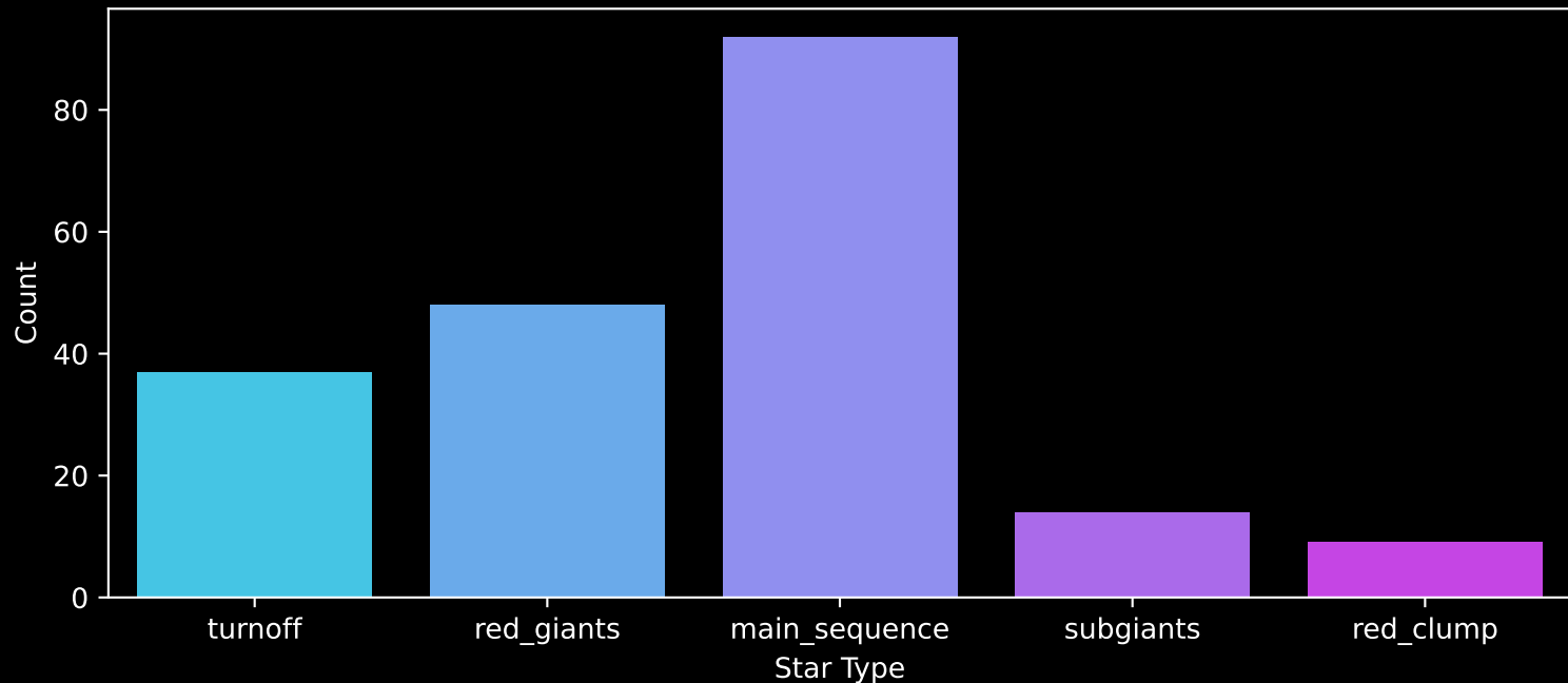
APOGEE DR17 Field: [267-32-O_TESS] Count plot of Star Type
