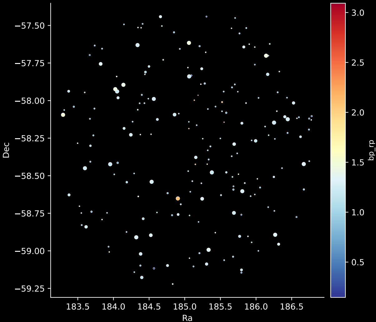
APOGEE DR17 Field: [267-32-O_TESS] Stars: 200
