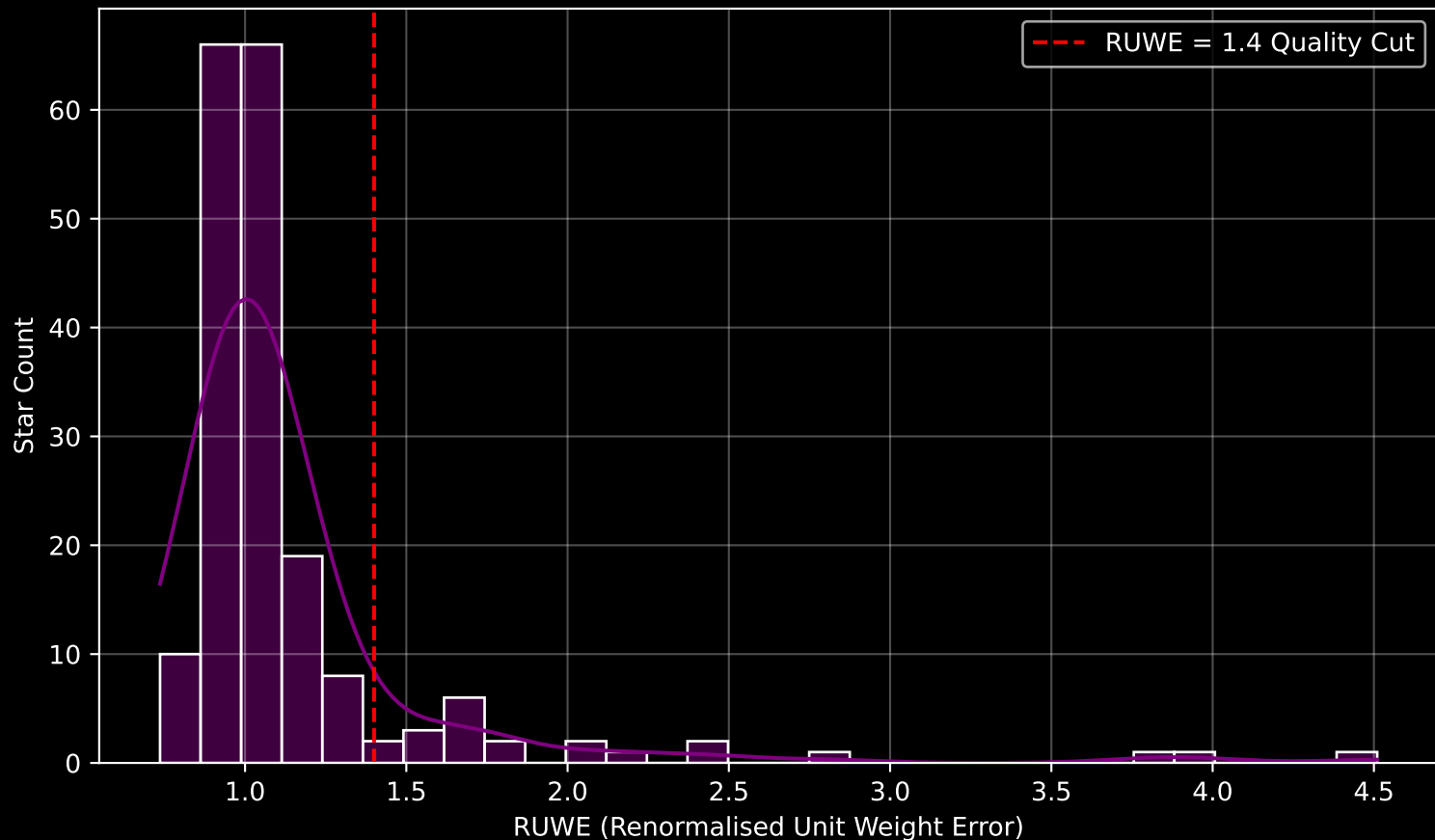
GAPOGEE DR17 Field [267-32-O_TESS] RUWE Distribution (n= 191)
